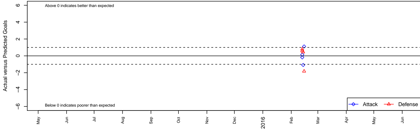
Croatian Eagles Red B97 Dots are actual minus expected GF (blue circles) and GA (red triangles). Blue line is smoothed change in attack strength. Red is smoothed change in defense strength.
